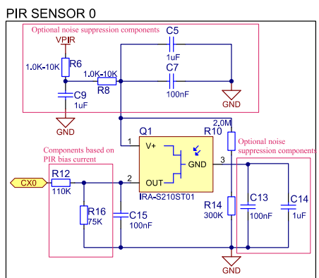
Figure 4-2: IQS62x and IRA-S210ST01
