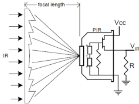
Figure 5-1: PIR Fresnel Lens
