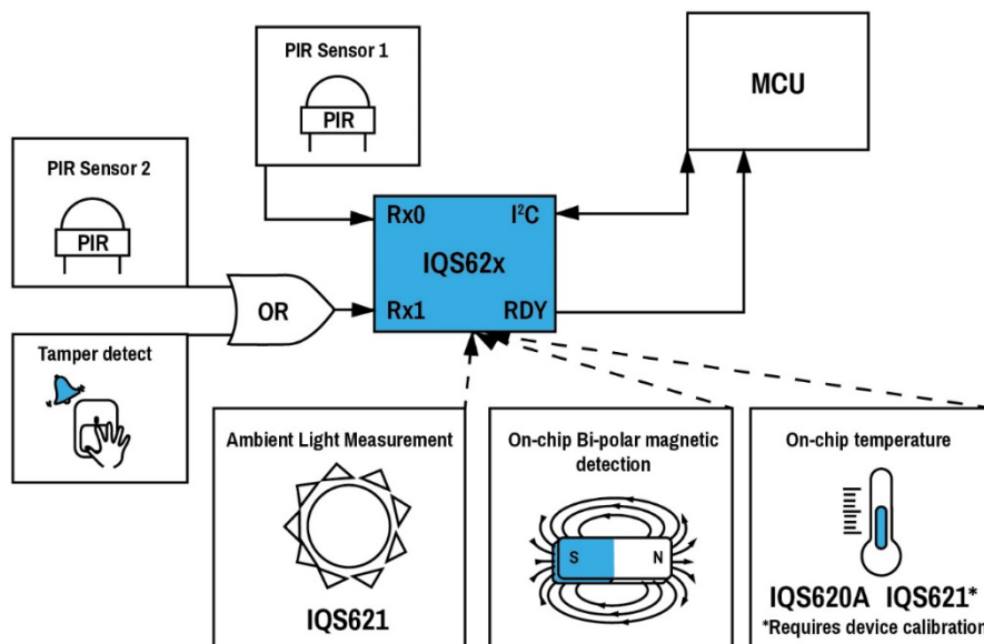
Figure 3-1: IQS62x Multifunctional PIR Sensor
