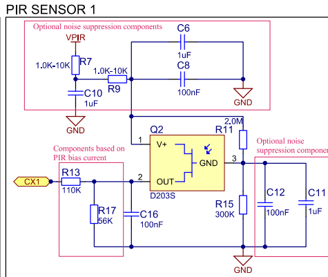
Figure 4-1: IQS62x and D203S (SENBA Optoelectronic)
