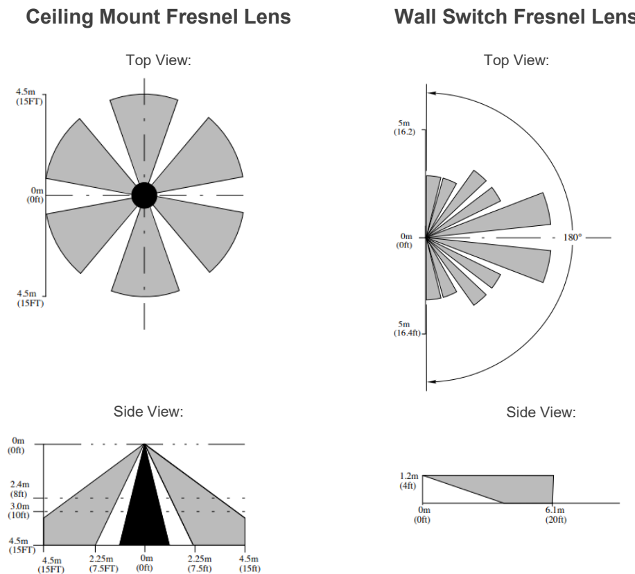
Figure 5-2: Different Fresnel Lenses (Adapted from: www.fresneltech.com )
