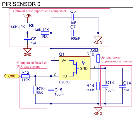
Figure 4-1: IQS62x and D203S (SENBA Optoelectronic)
