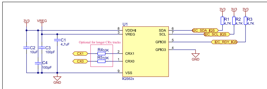
Figure 4-1: IQS62x and D203S (SENBA Optoelectronic)
